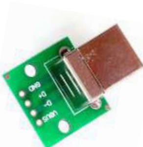
T1091 USB Type B Female Socket Breakout Board 2.54mm Pitch Adapter Connector
