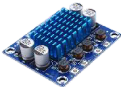
T1051 XH-A232 TPA3110 30W+30W 2.0 Channel Digital Stereo Audio Power Amplifier Board
