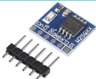
T1061 W25Q32 Large Capacity Flash Storage Module
