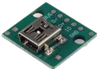
T1089 USB To DIP 2.54mm Female B Type Patch To Invert Adapter Board
