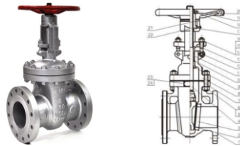
11C API 600 WEDGE GATE VALVES
