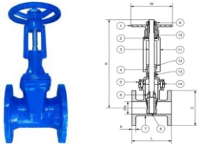
11A SANS 665 / BS 5163 PN16 RESILIENT SEAL GATE VALVES
